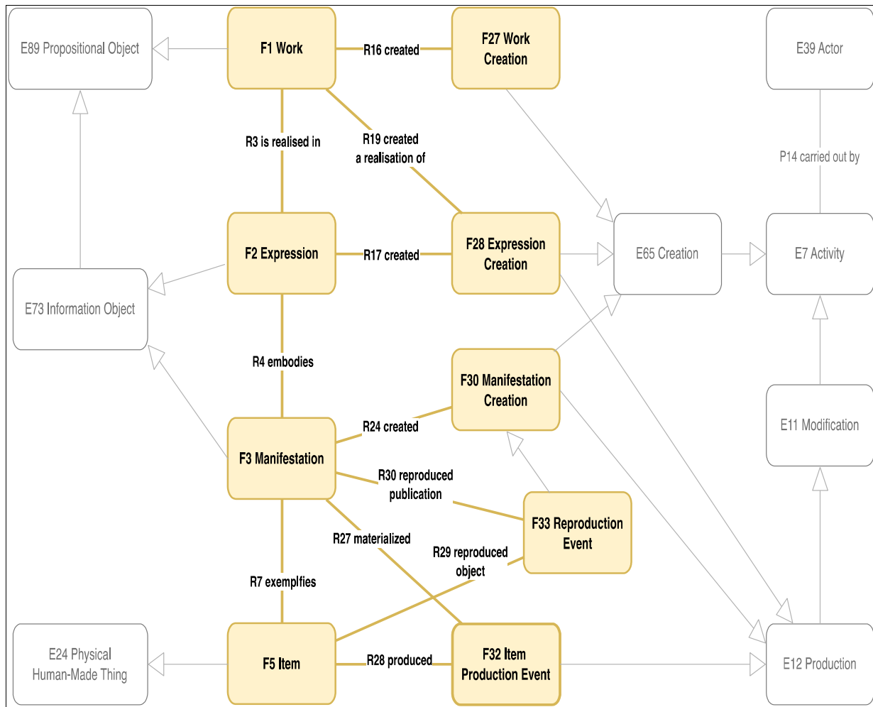
Illustration 1. LRM 00 classes and properties and their connections to CIDOC CRM classes
