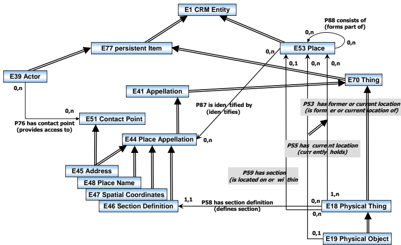
fig. 2 reasoning about spatial information
