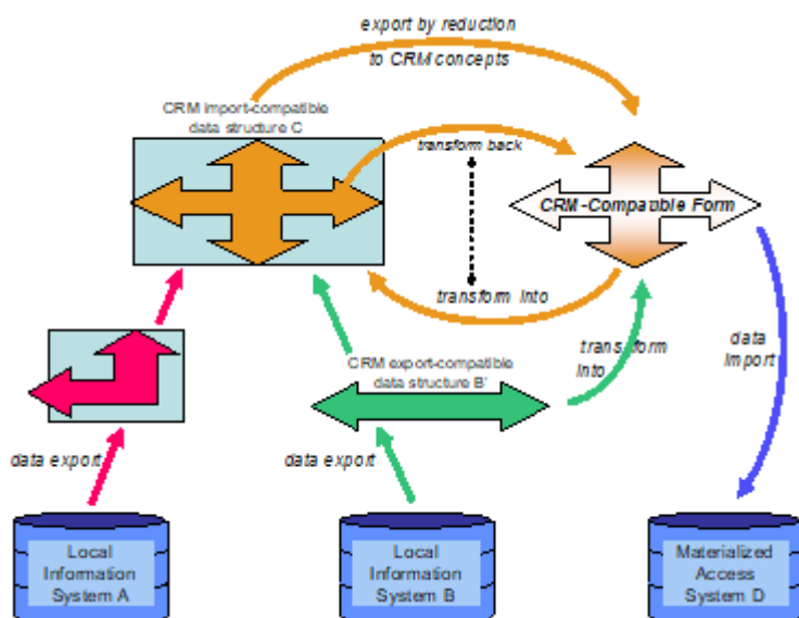
fig. 1: Possible data flow between different kinds of CRM-compatible systems and data structures Definition of the CIDOC Conceptual Reference Model version 6.2.3 E.S.: In Progress since [17/5/2018]
