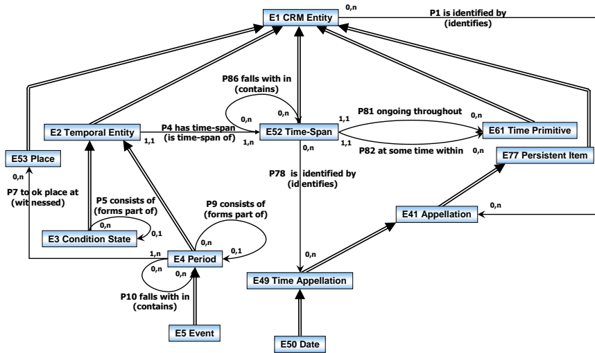
fig. 3 reasoning about temporal information
